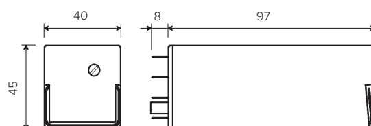
Relay with flat head slotted screw setting control
